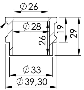
"S.S. Bushing" Cod.206442
